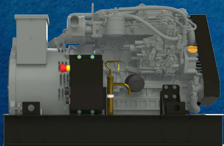
With Base Frame
