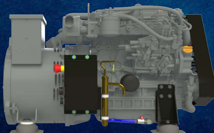
Base Frame Removed
